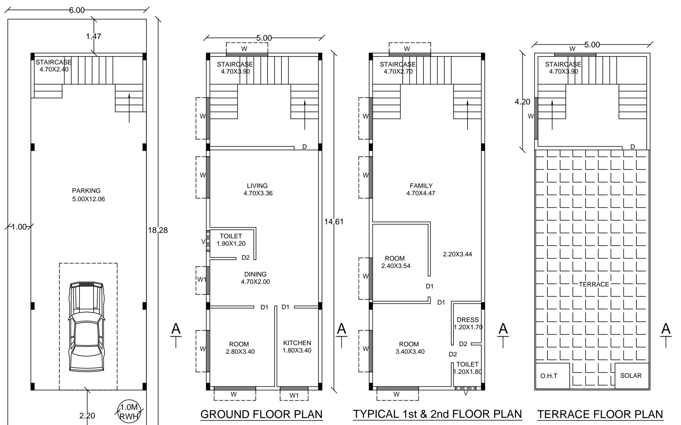
STILT FLOOR PLAN
